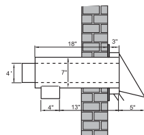
FT-4 Concentric Pipe-in-Pipe Termination
