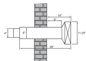
AT-4 Aerocowl Termination
